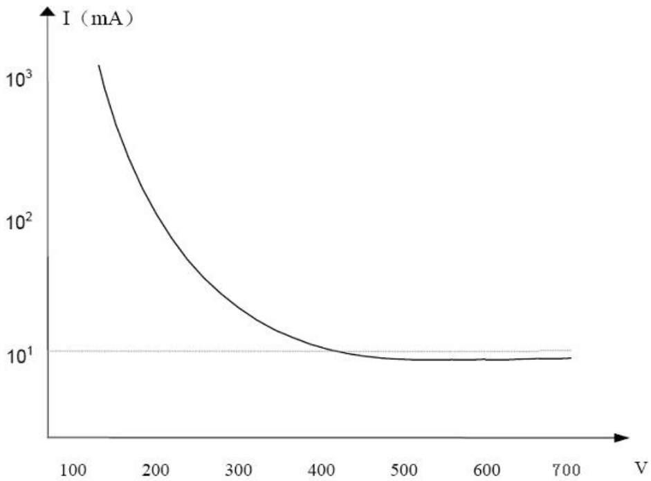
参考曲线 Curve of reference
